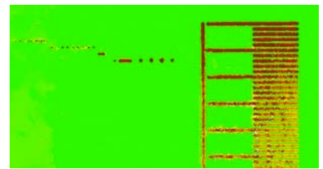
C-Scan Side Arm Pipe OD \geq 3"
